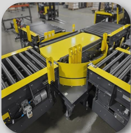
TURN TABLE
