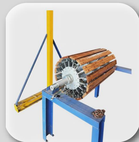
FORMER (MANDREL)
